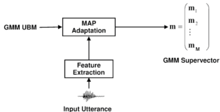
Figure 3. Gaussian suprvector formulation [13].
