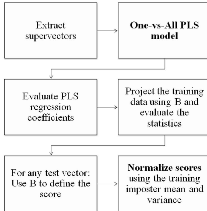
Figure 5. GSV-PLS training and testing block diagram [4].
